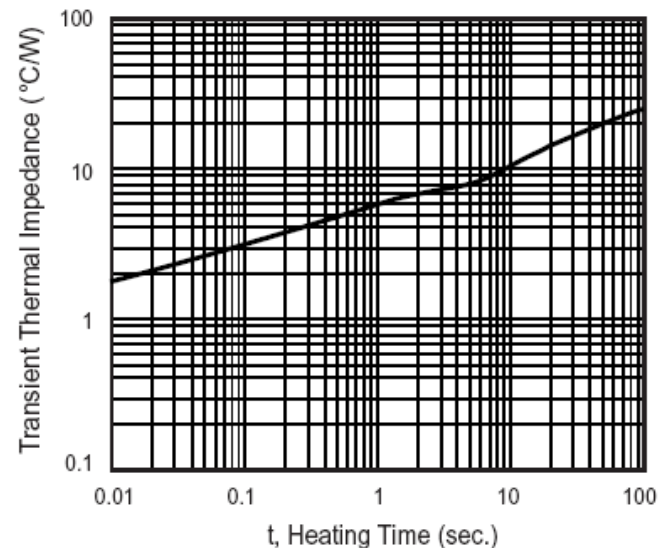
Figure 6. Typical Transient Thermal Impedance Per Leg
