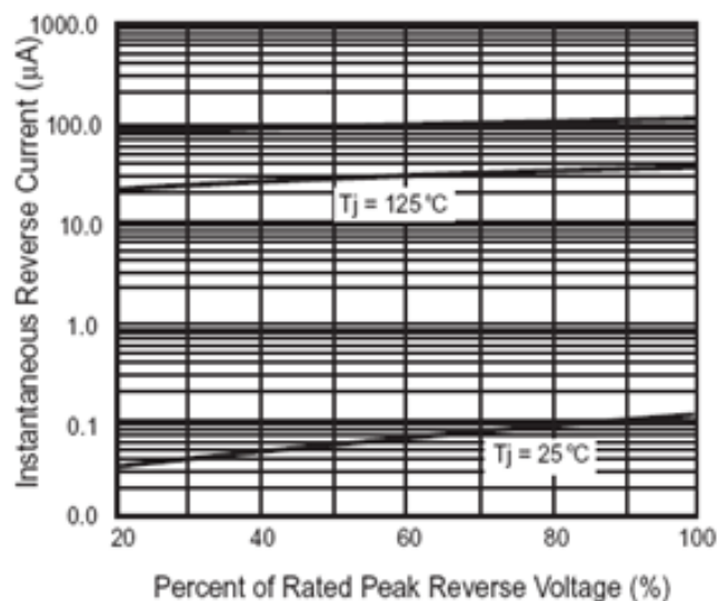
Figure 4. Typical Reverse Characteristics Per Leg
