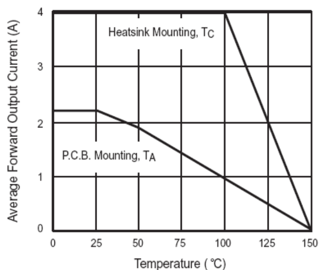
Figure 1. Derating Curve Output Rectified Current
