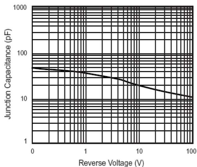
Figure 5. Typical Junction Capacitance Per Leg
